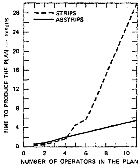
FIG. 5. Planning time as a function of plan length.
