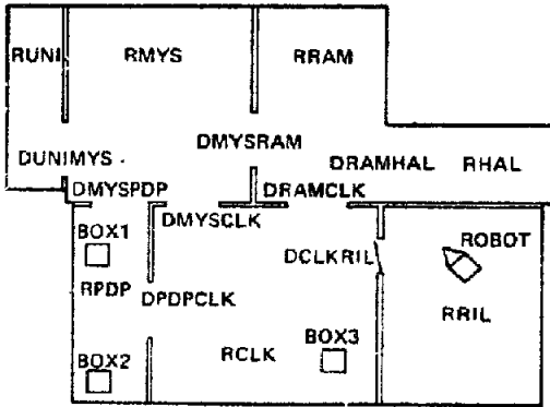
FIG. 2. Initial state for the sample problem.
